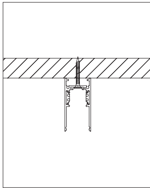
Deep Ceiling Mounted
