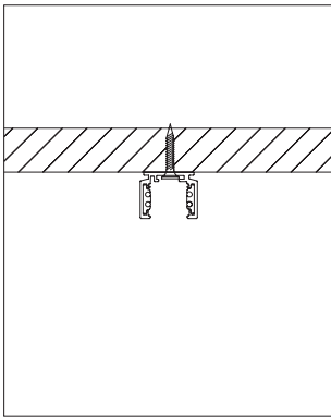
Ultra-thin Ceiling Mounted
