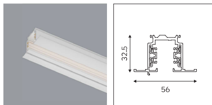
3 Circuit Track (Recessed) 1M/1.5M/2M/3M Length Cut-out: 35mm
