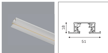
1 Circuit Track (Recessed) 1M/1.5M/2M/3M Length
