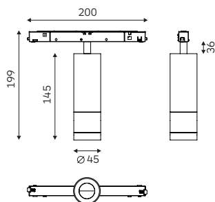
FEEL ZOOM 45 Low Voltage Track
