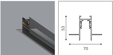
Low Voltage MagneticTrack Recessed 1M/1.5M/2M/3M Cut-out: 28mm
