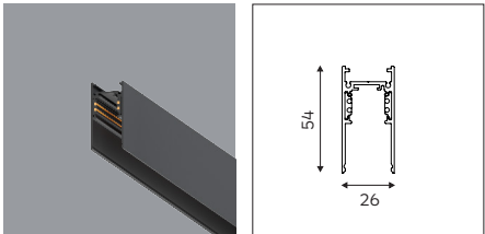
Low Voltage Magnetic Track Ceiling Mounted and Pendant 1M/1.5M/2M/3M
