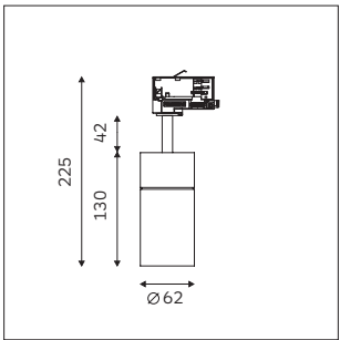
EMMA 62 Body Sizes: Ø62XH130mm Body Material: Aluminum/Iron Color: White/Black Optic: Lens
