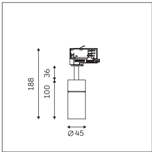
EMMA 45 Body Sizes: Ø45XH100mm Body Material: Aluminum/Iron Color: White/Black Optic: Lens
