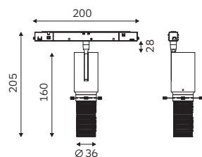
ARTAX 45 Low Voltage Track
