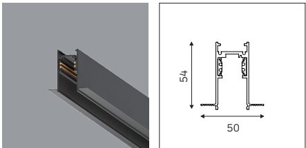
Low Voltage Magnetic Track Recessed 1M/1.5M/2M/3M Cut-out: 28mm
