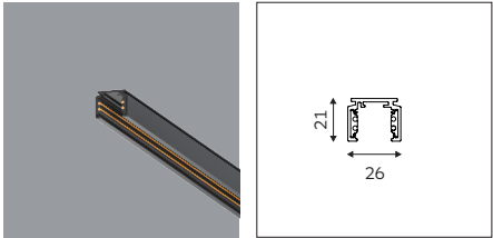
Low Voltage Magnetic Track Ultra-Thin Ceiling Mounted 1M/1.5M/2M/3M
