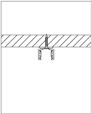
Ultra-thin Ceiling Mounted
