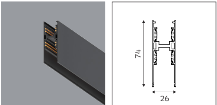
Low Voltage Magnetic Track Pendant 1M/1.5M/2M/3M
