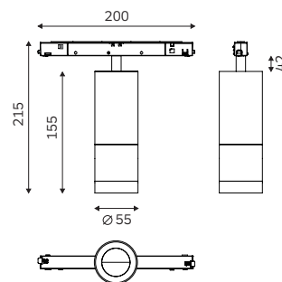
FEEL ZOOM 55 Low Voltage Track
