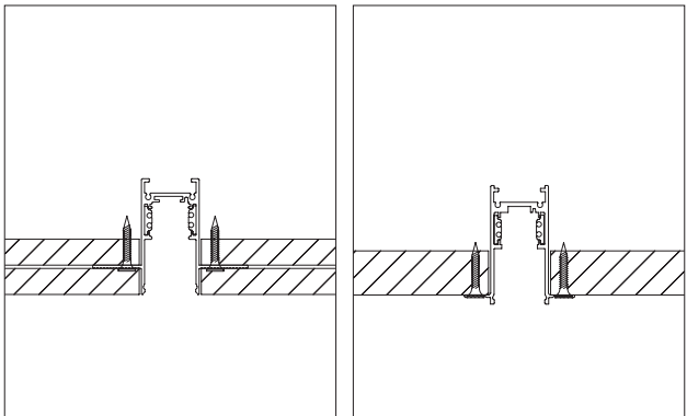
Two-Wood Recessed Trimless Recessed
