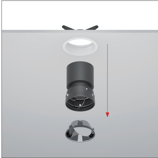
4. A pull ring allows the luminaire to be pulled down by hands without any tooling, providing great convenience for the maintenance of the luminaire
