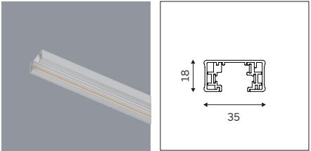
1 Circuit Track (Ceiling Mounted) 1M/1.5M/2M/3M Length
