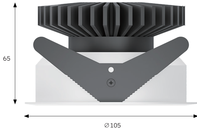
UTH 95 Cut-out: Ø95mm Power: 14.3W Optic: Lens
