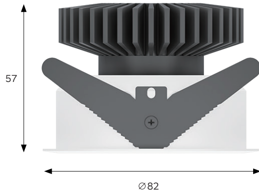
UTH 75 Cut-out: Ø75mm Power: 8.6W Optic: Lens
