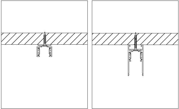
Ultra-thin Ceiling Mounted Deep Ceiling Mounted
