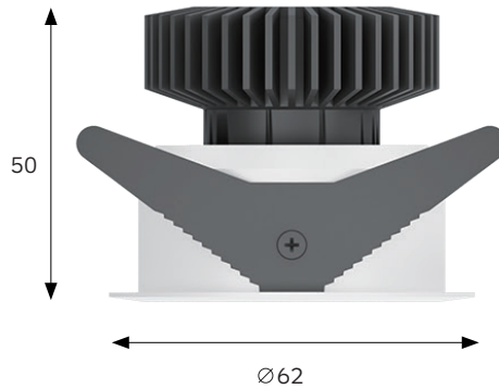
UTH 55 Cut-out: Ø55mm Power: 7W Optic: Lens
