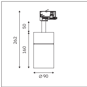
EMMA 90 Body Sizes: Ø90XH160mm Body Material: Aluminum/Iron Color: White/Black Optic: Lens
