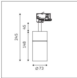
EMMA 73 Body Sizes: Ø73XH148mm Body Material: Aluminum/Iron Color: White/Black Optic: Lens
